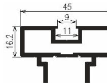
SLP-HP-4516 Horizontal [ 16x45 ]
